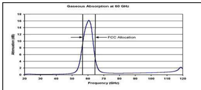
Fig 5. Oxygen Attenuation vs. Frequency
