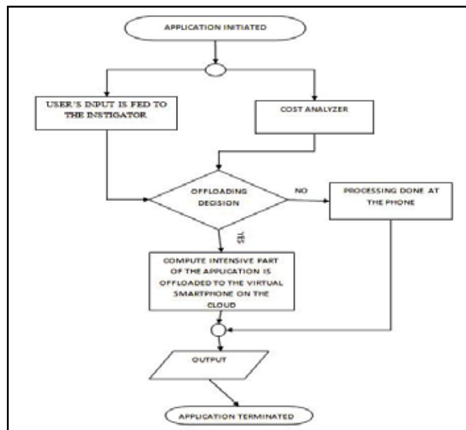
Fig. 4: Control Flow Diagram of the Proposed Framework
