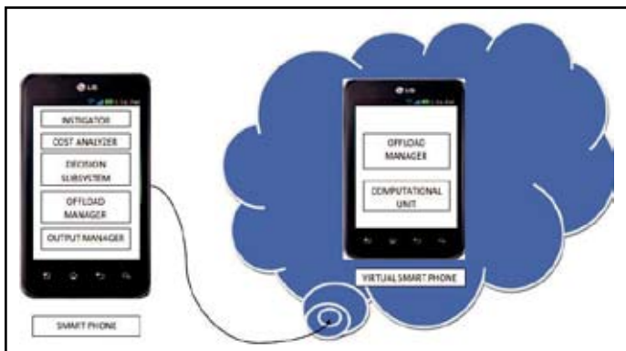
Fig. 3.: Framework of Autonomous Computation Offloading Application for Android Phones.
