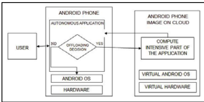
Fig. 2 : Overview of Autonomous Computation Offloading Application for Android Phones.
