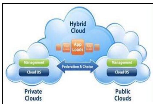
Fig 3: Cloud Types
