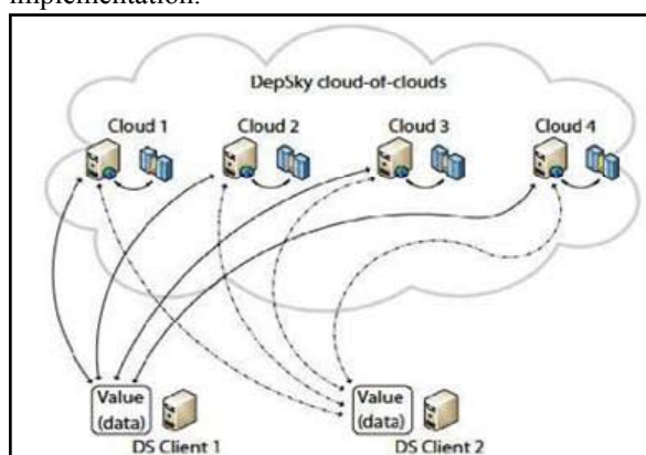
Fig 5: DepSky Architecture
