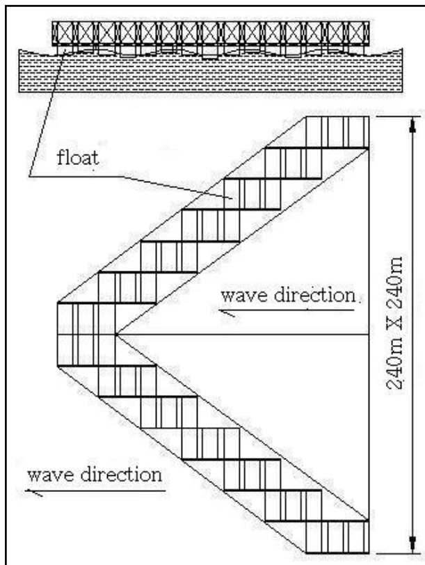
Fig. 2 : Wave Power Device
