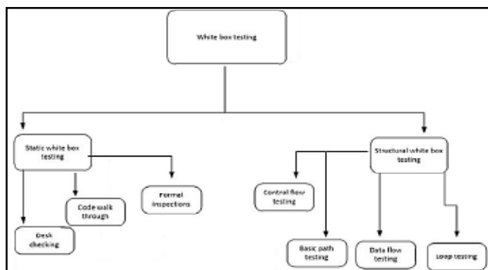
Fig. 2 : Different forms of White Box Testing
